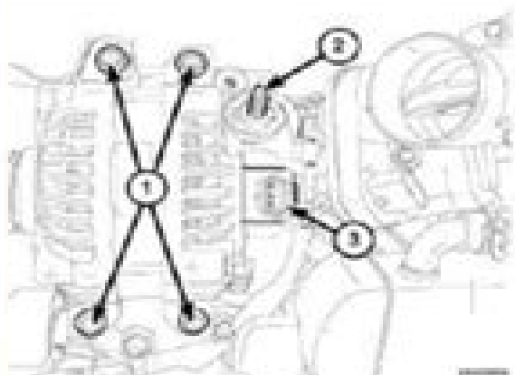
Fig. 9: Generator Belt & Connector Courtesy of CHRYSLER GROUP, LLC
