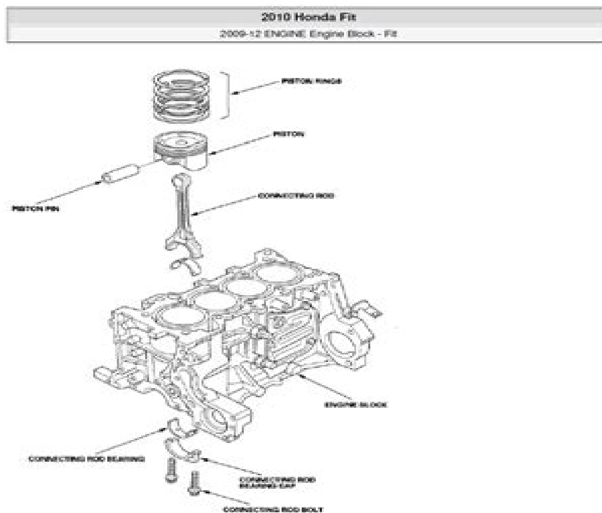
Fig. 3: Identifying Engine Block Replacement Components (2 Of 2)
