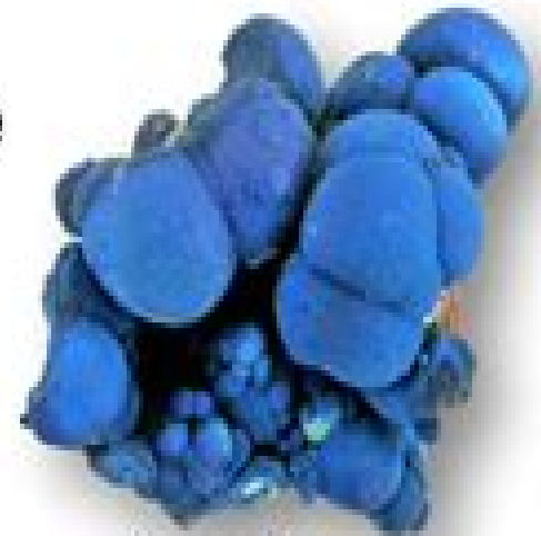
Azurite \text{Cu}_3(\text{CO}_3)_2(\text{OH})_2
