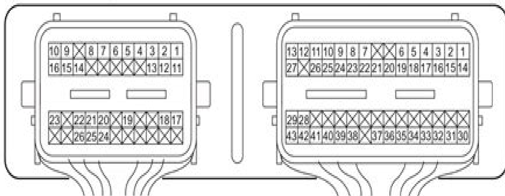
[A]: ECM connector (View: A)
