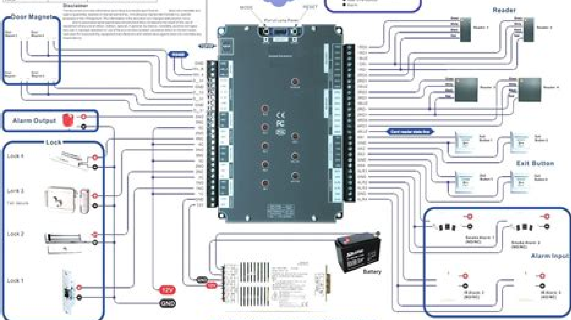
Wiring Diagram of Access Controller
