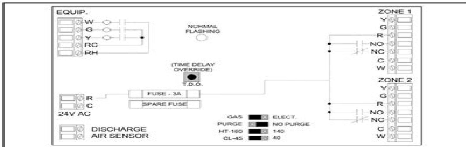
FIGURE 1 – LENNOX® MODEL LZP-2 CONTROL PANEL LAYOUT
