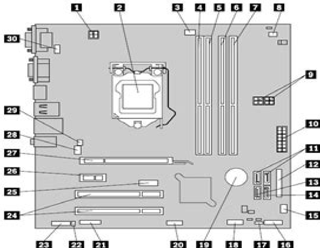
Figure 4. System board part locations
