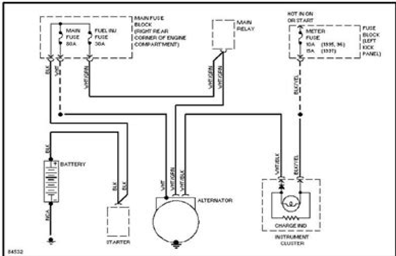
Charging Circuit
