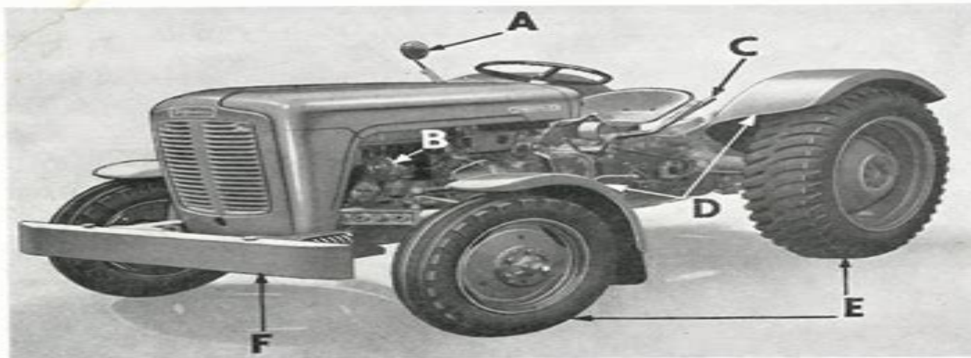
FIG. 1. INDUSTRIAL TRACTOR
