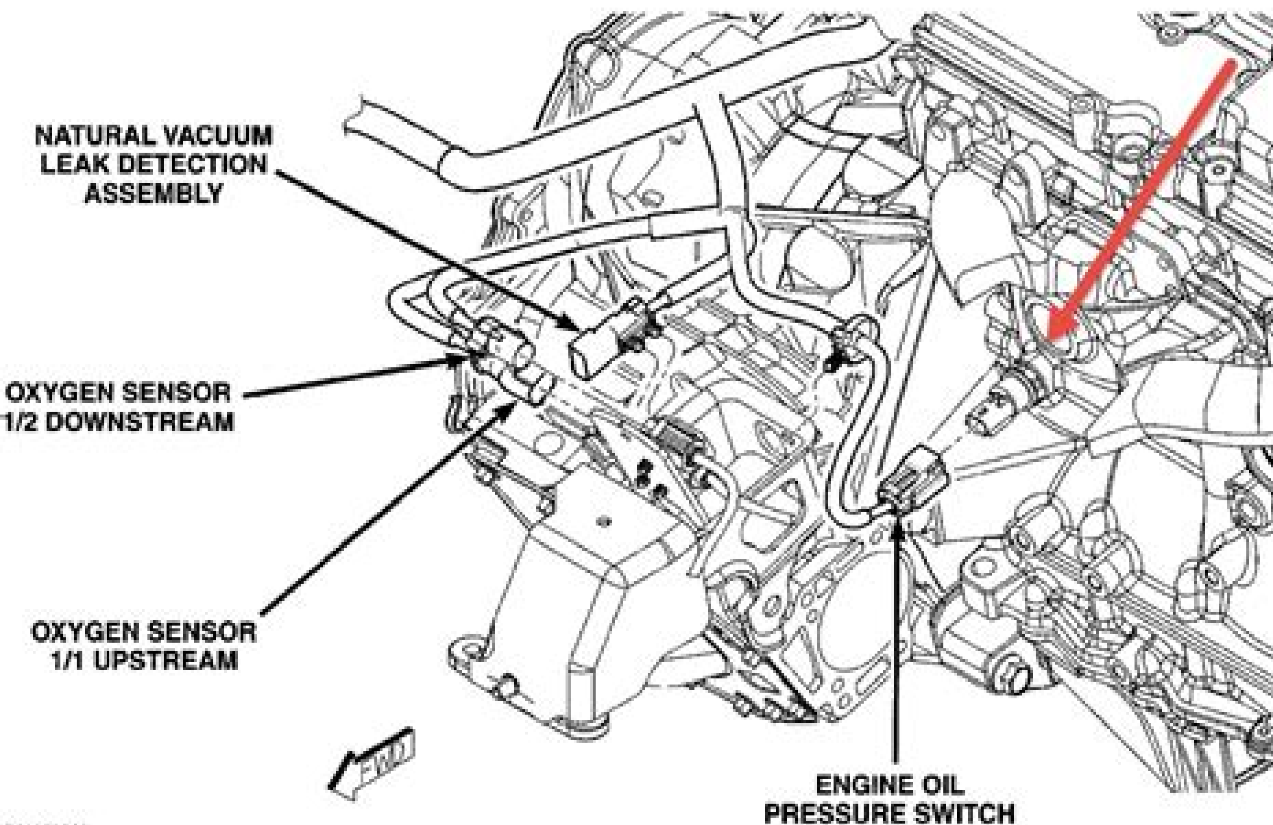
Fig. 1: Right Side Of Engine (2.4L)
