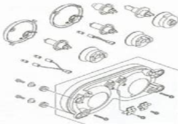
9.3a Headlight assembly details
