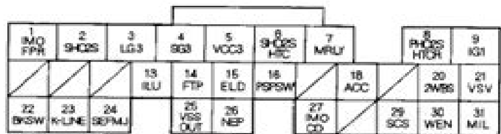
Wire side of female terminals
