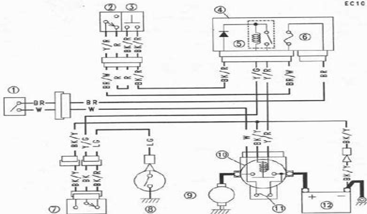
Electric Starter Circuit
