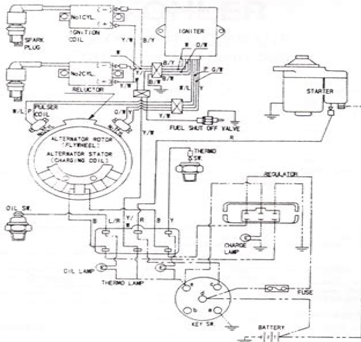
518-Engine wiring diagram.
