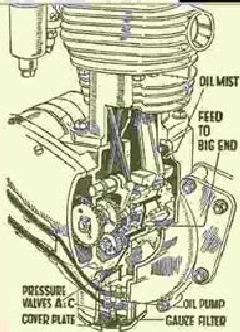
Fig. 3: Lubrication System, Model C11
