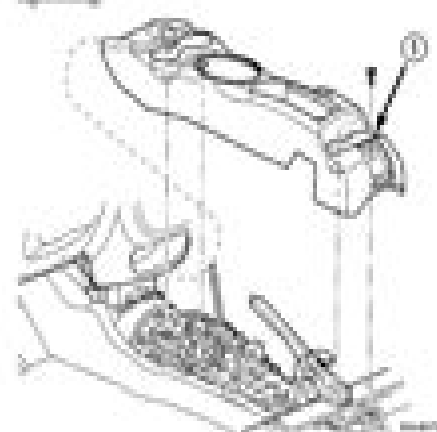
Fig. 160 Center Console Removal/Installation - Detail
