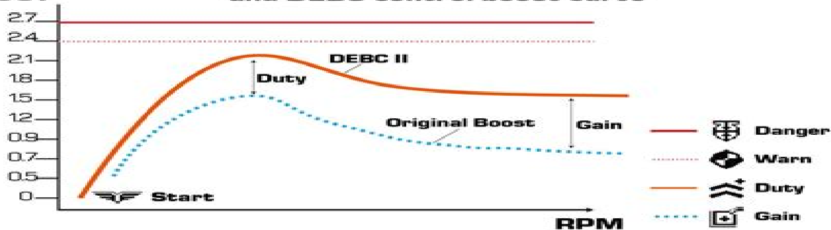
Schematic diagram of original turbocharging and DEBC control boost curve
