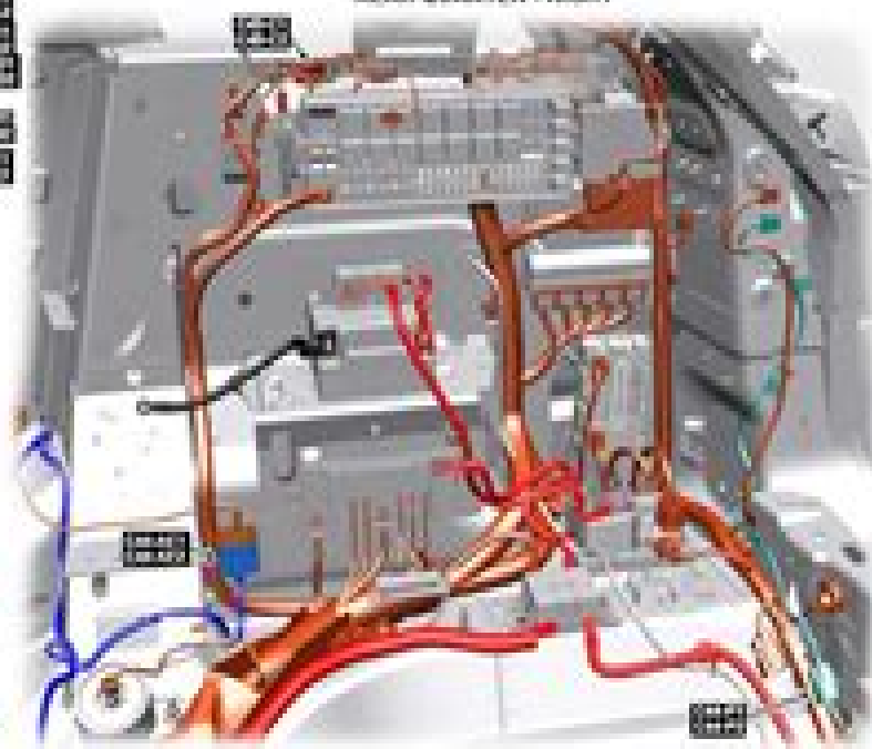
AREA 'I' REAR QUARTER - RIGHT
