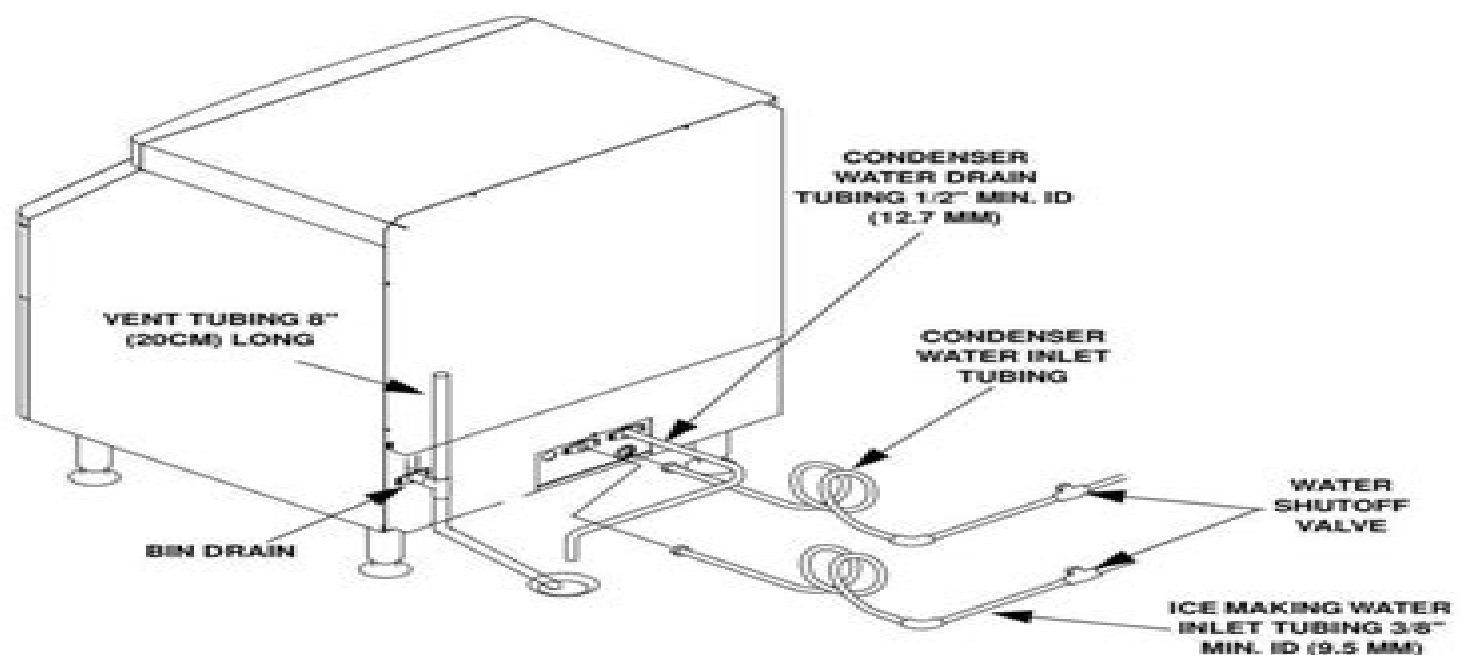
Typical Water Supply Drain Installation
