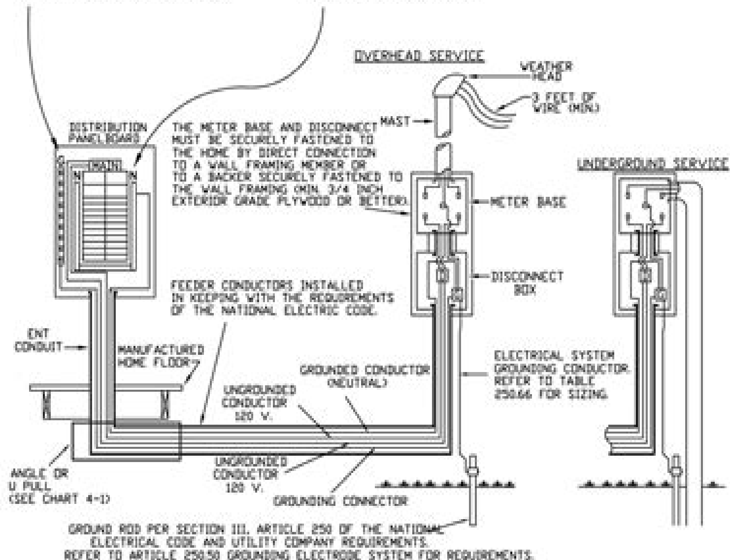
TYPICAL FEEDER MAKEUP & GROUNDING (ABOVE GROUND)
