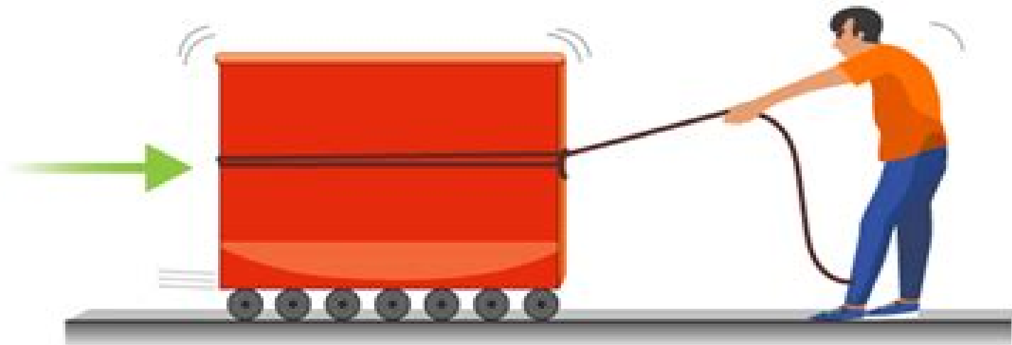
Rolling Friction
