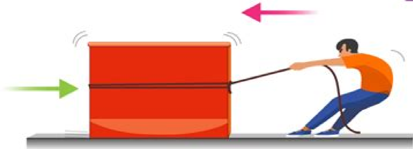
Sliding Friction
