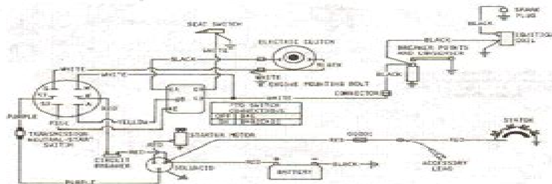
Fig. JD141—Electrical wiring diagram for Models 108 and 111 tractors (S.N. 95001-120000).
