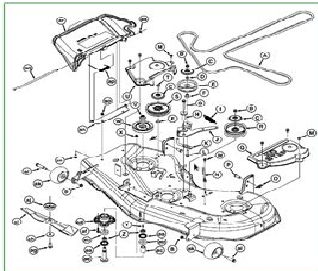
MXT004905-UN: Deck Spindles and Sheaves 54C
