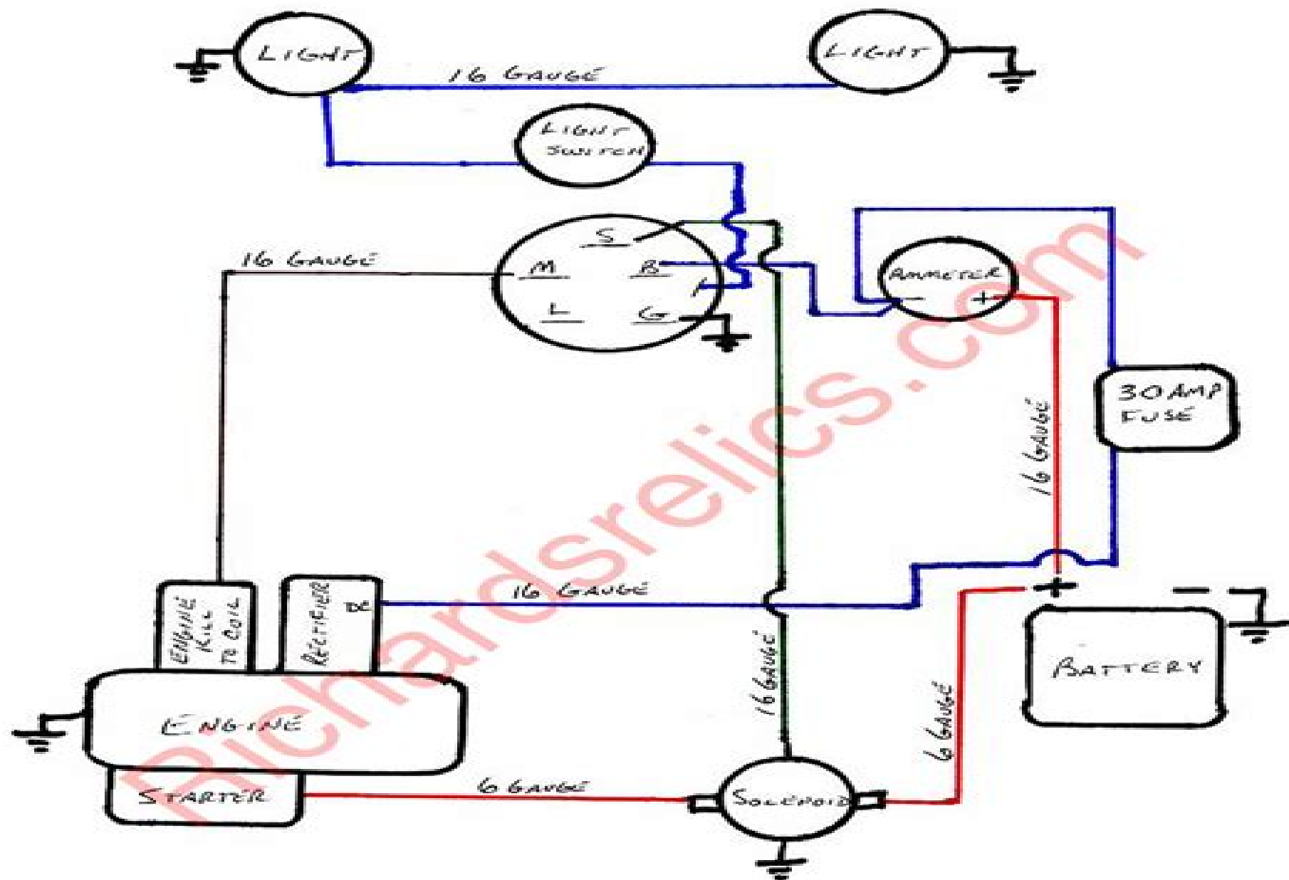
HUSTLER BRIGGS & STRATTON 18HP WIRING IGNITION SWITCH 3 POSITION #399
