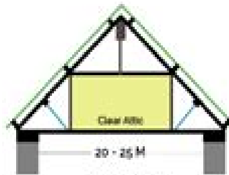
Attic Truss
