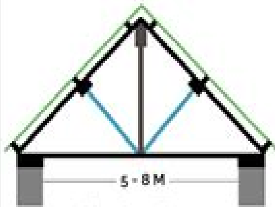
King Post Truss
