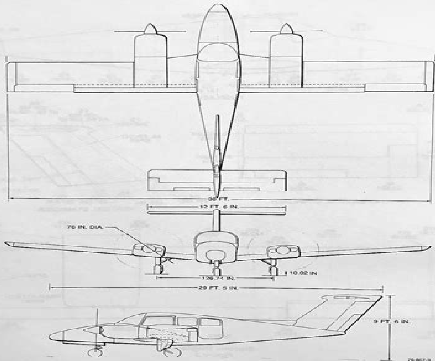
Airplane Dimensions Figure 1
