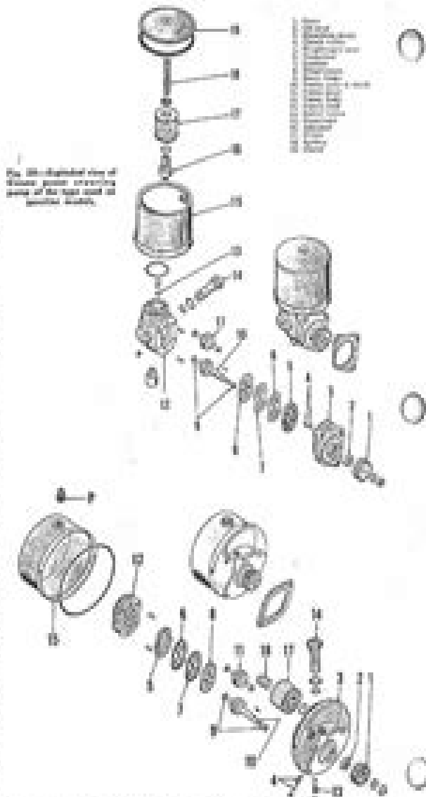
Fig. 21—Exploded view of steering pump assembly showing the pump, drive shaft, and various seals and components.
