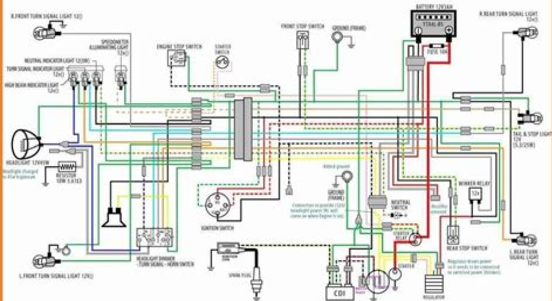
ENGINE STOP SWITCH ARRANGEMENT
