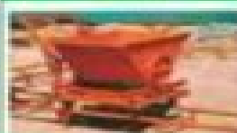
Slab Trolley Capacity 7 CFT Rail- 150 FT & 2 Barred (40 mm dia)
