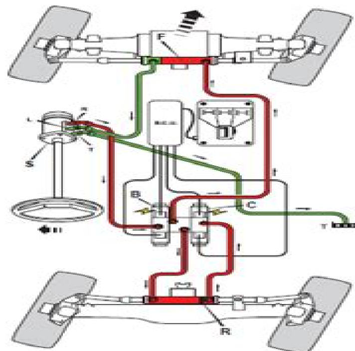
Fig 5. Typical Machine with Power Track Rods - Right turn shown
