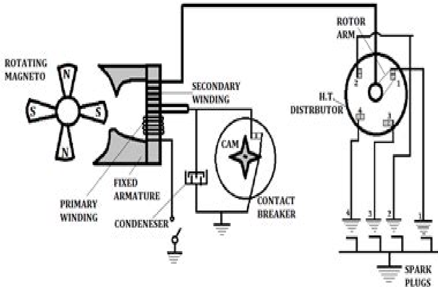
FIG: MAGNETO IGNITION SYSTEM
