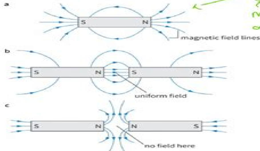
Figure 24.2: Magnetic field patterns: a for a bar magnet; b for two attracting bar magnets and c for two repelling bar magnets.
