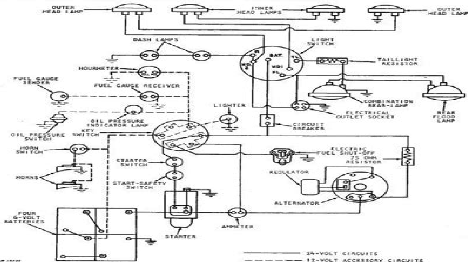
Fig. 150-10-1—Schematic Diagram of the Electrical System
