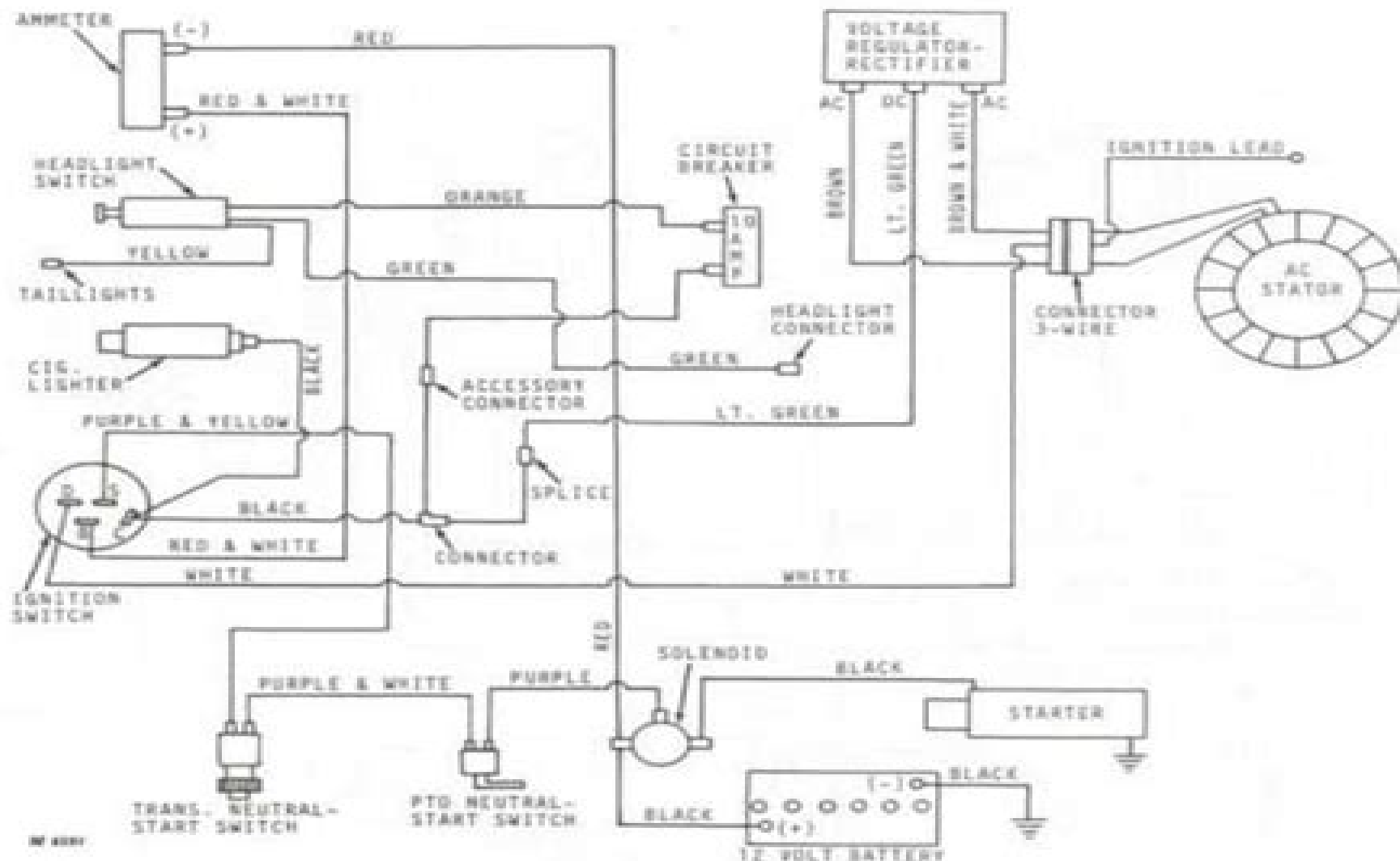
Fig. 3-AM32174 Wiring Harness with AM30771 Ignition Switch with Headlights and Lighter, Tractors (Serial No. 100,001-130,000)
