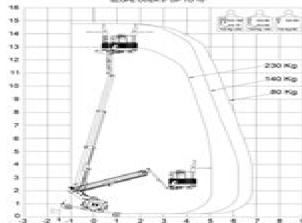
J888 1450 (21V)-LTH WORKING DIAGRAMS LATERAL SIDE SLOPE OVER 15° UP TO 18°
