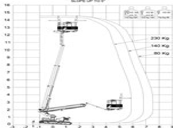
J888 1450 (21V)-LTH WORKING DIAGRAMS LATERAL SIDE SLOPE UP TO 15°
