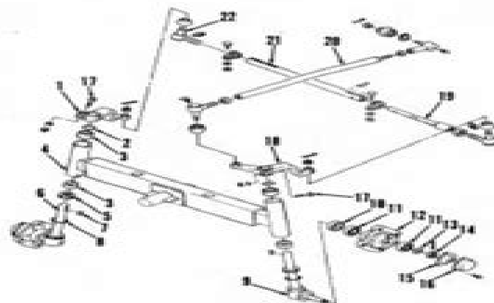
Fig. 5—Exploded view of steering spindles, wheel hub and steering linkage used on late Model MT210 (after serial number 70765) and all Model MT250 tractors. Early Model MT210 tractors are similar except axle thread which is not adjustable.
