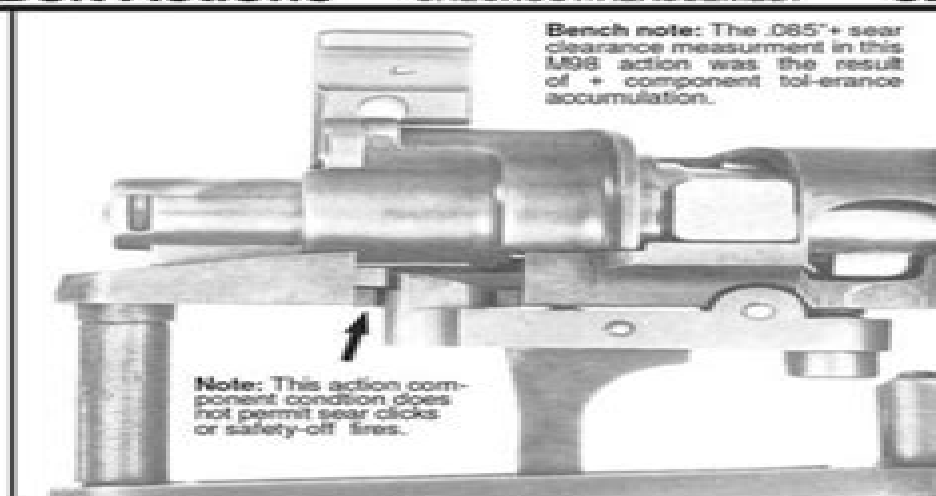
Figure 47- Shows a cocking piece in a cutaway M98 action set back by rotating the safety lever to disassembly position . Cocking piece ledge/trigger sear clearance is .085" + in this action. In serviceable M98 actions, sear clearance is typically the same in both the safety and disassembly detents. In the safety lever disassembly position the bolt can be cycled to check both sear engagement and clearance.
