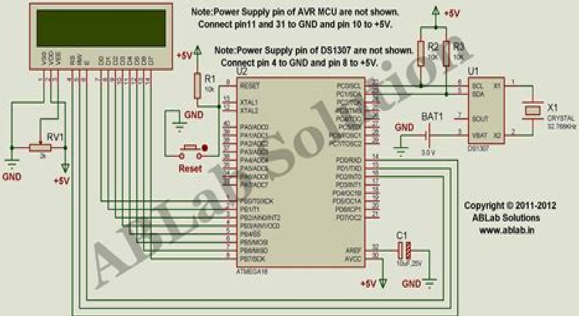
Circuit Diagram of DS1307 RTC Interfacing with ATmega16 and LCD Display
