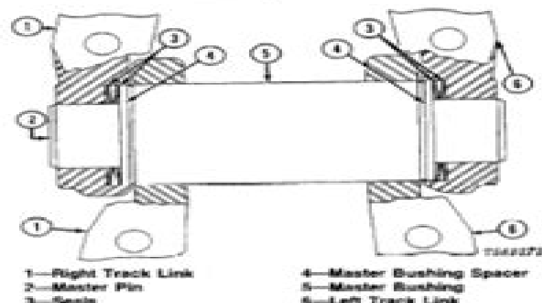
Fig. 19-Master Pin Connection Seal Placement
