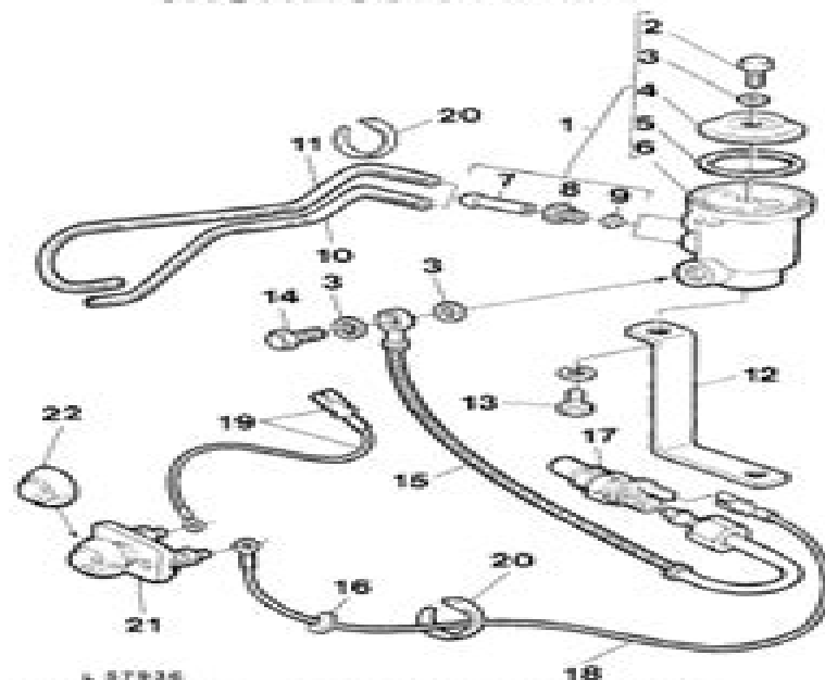
Fig. 2 — "Thermostart Aid", Exploded View
