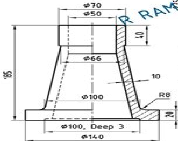
BODY (CAST IRON)
