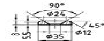
SPECIAL WASHER (MILD STEEL)
