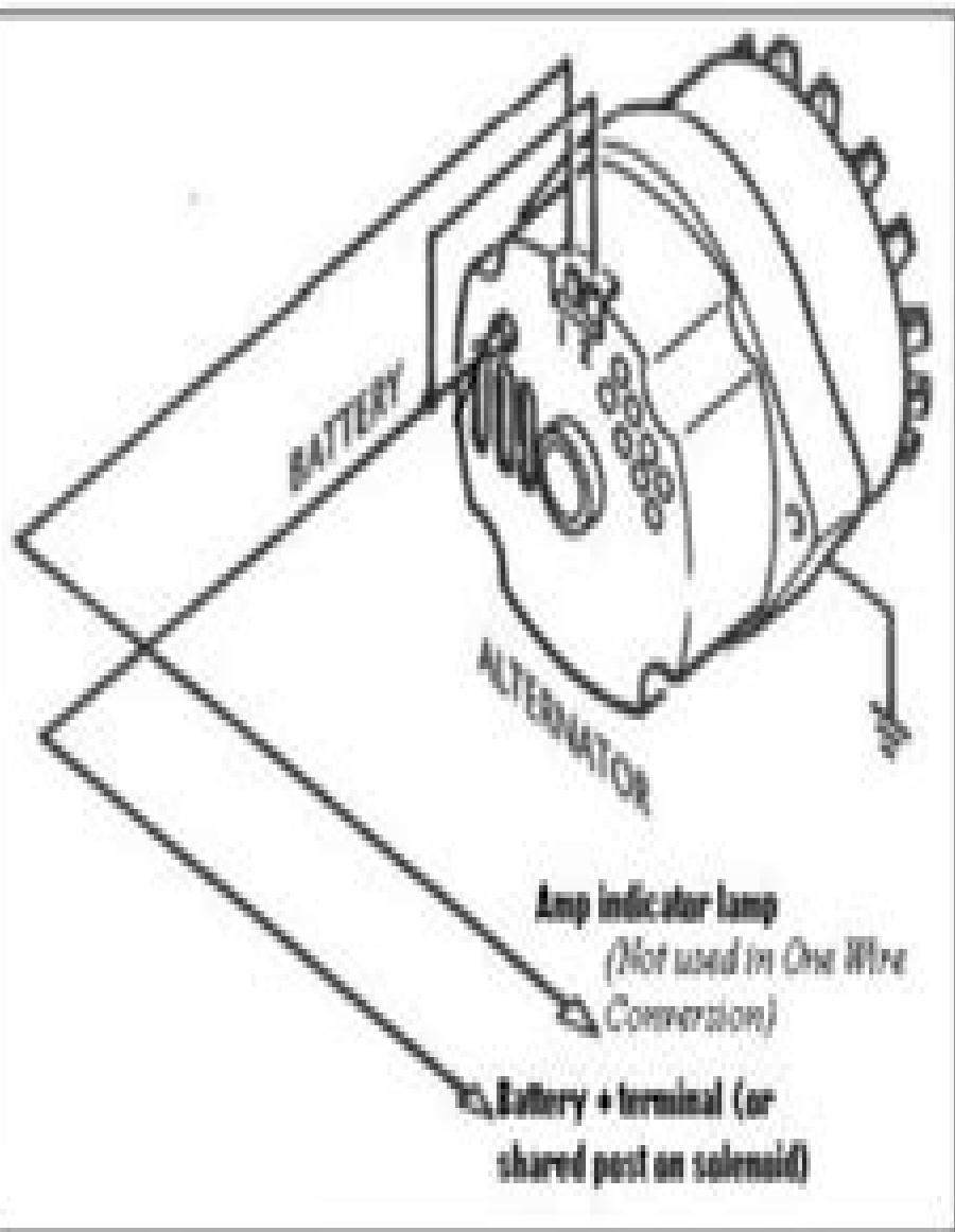
Delco Alternator (Internal)
