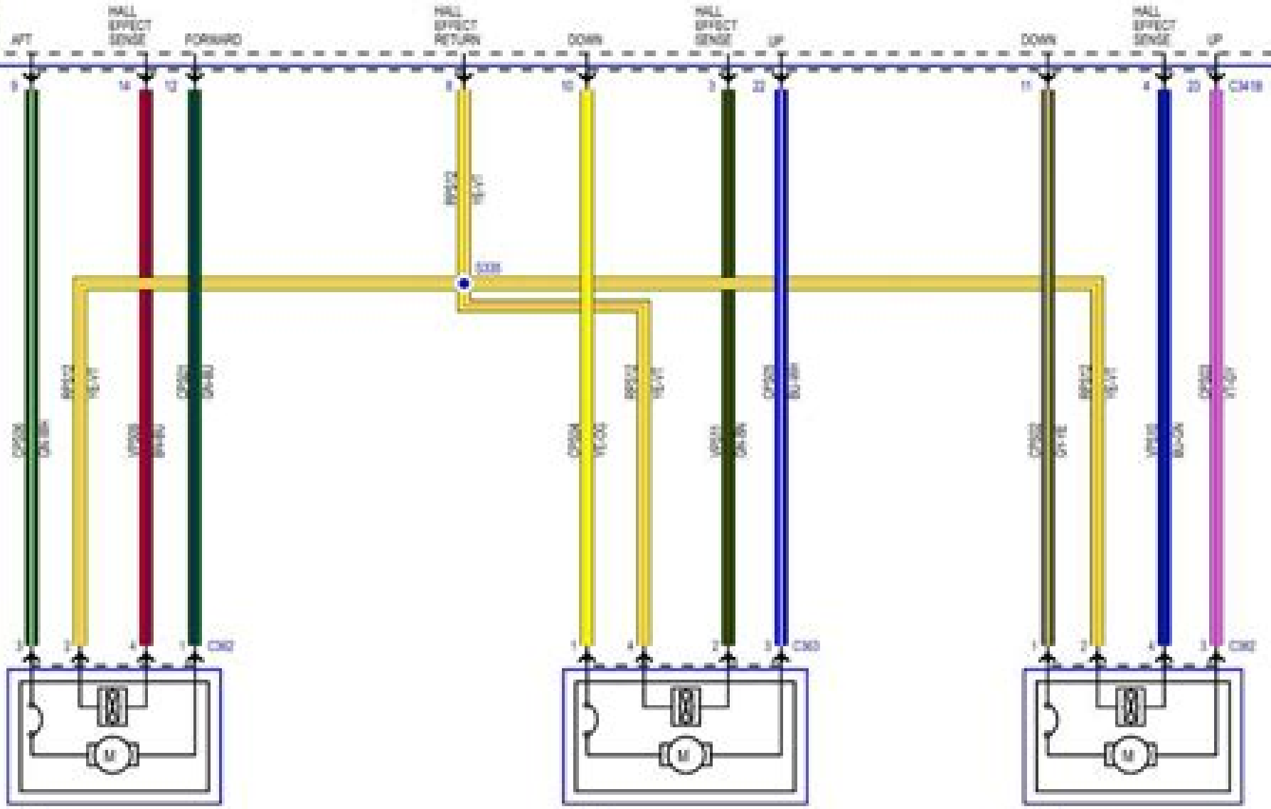
FRONT SEAT TRACK MOTOR LH
