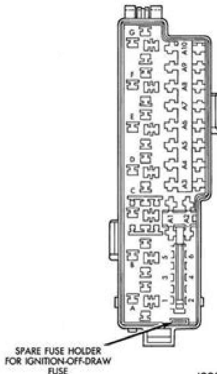
Fig. 15 Power Distribution Center
