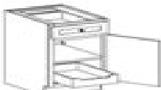
Base Single Door w/Deluxe Full Width Tray (B) - (#216/T) Available sizes: Width: 12, 15, 18, 21, 24 Depth: 24 Height: 34 1/2
