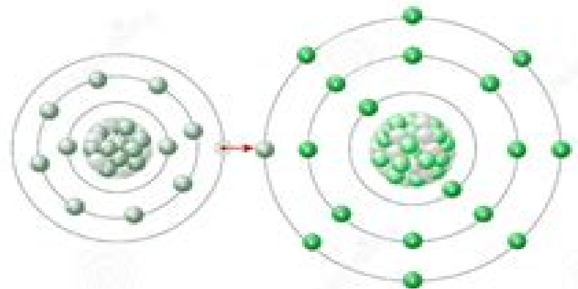
Ionic bond
