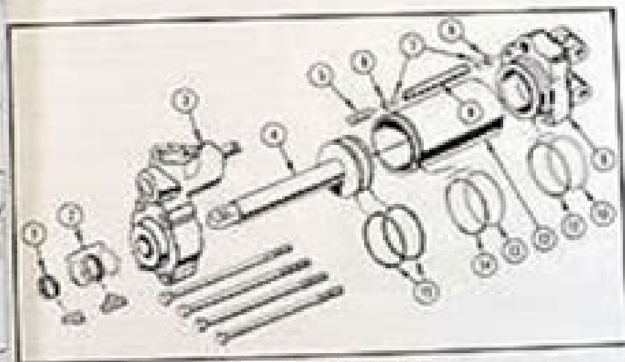
Fig. 14 - Exploded View of Valve Body
