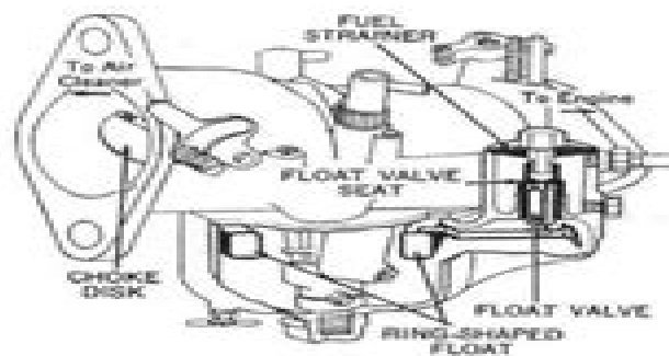
FUEL-CONTROL SYSTEM
