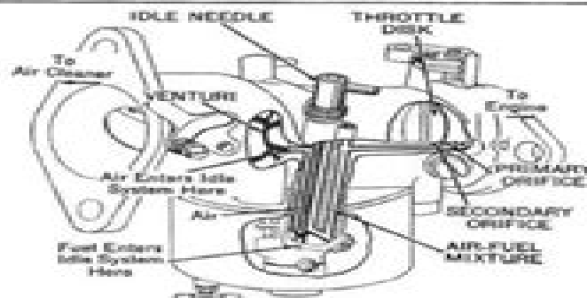
IDLE SYSTEM
