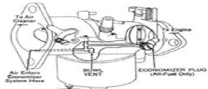
BACK-SUCTION ECONOMIZER SYSTEM
