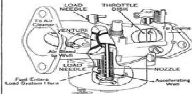
LOAD SYSTEM
