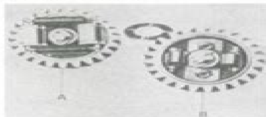
Fig. L25—Two types of gear driven flyweight governors are used on three cylinder engines. A constant speed "A" or a variable speed "B" governor is located within timing gear cover.
