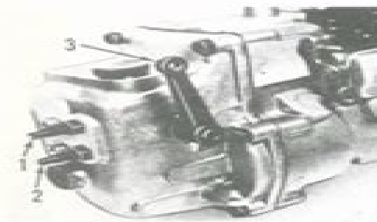
Fig. L24A—View of low and high speed adjusting screws located on rear of governor housing on Minimec pump. Refer to text for adjustment procedure.
