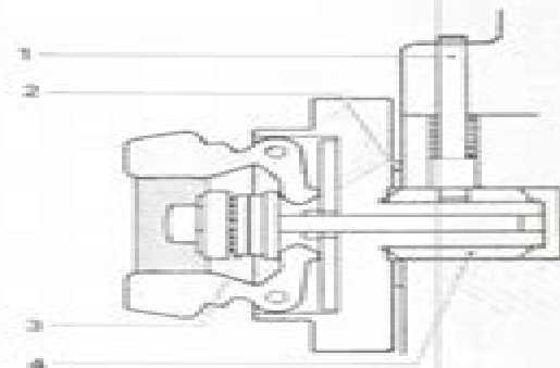
Fig. L26—Governor gear is driven directly by the camshaft and runs in a renewable bearing.
