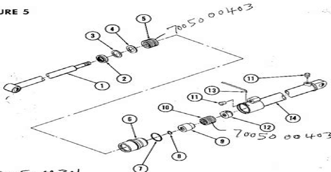
PARTS LIST Figure 5 — 1-3/4" Double Acting Lift Cylinder Part No. 7713
